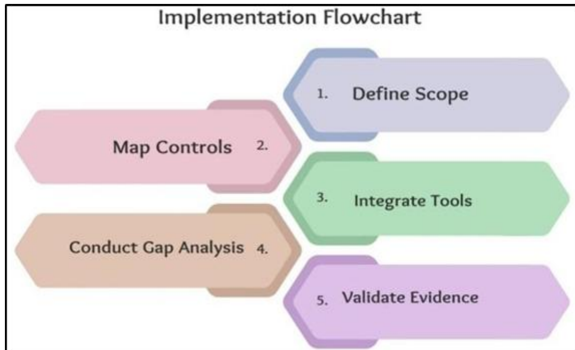
Fig 4. Implementation Flowchart
